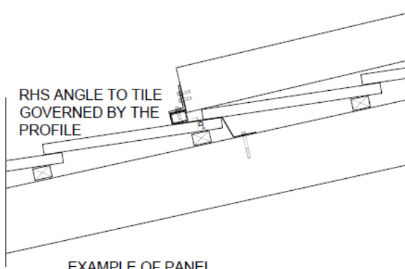
EXAMPLE OF PANEL FIXING AT THE BOTTOM
