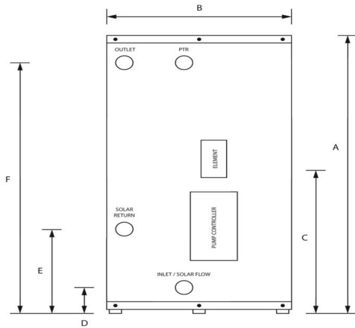
ROUGH IN PIPEWORK DIMENSIONS (mm)
